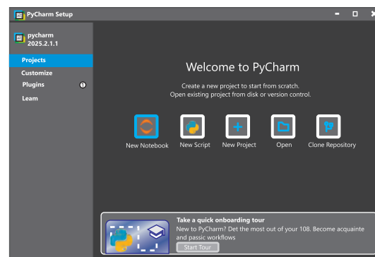
Figure 2.4: Python IDE
