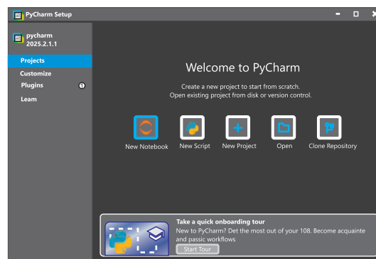
Figure 3.4: Python IDE
