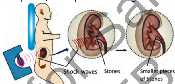
Figure 5.3: Lithotripsy
