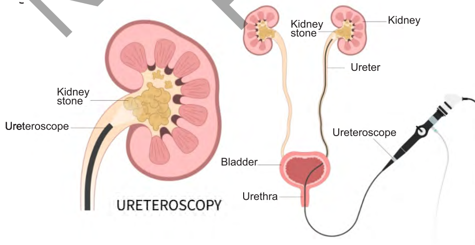
Figure 5.4: Ureteroscopy
