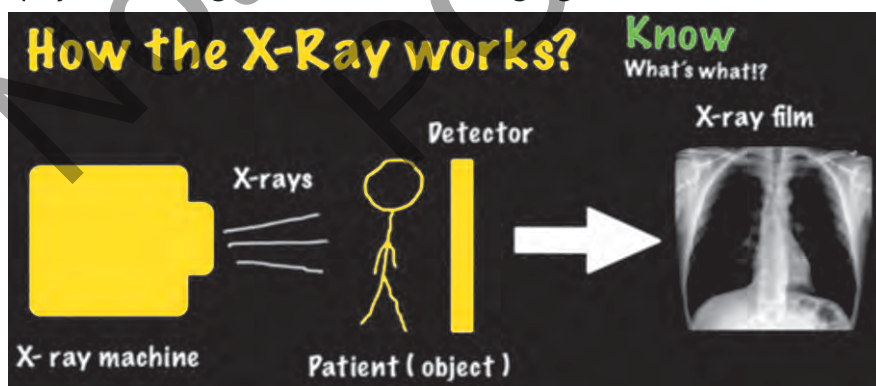
Figure 3.3: X-ray
