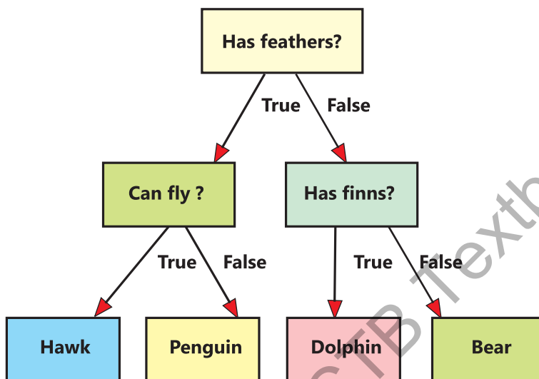
Figure 8.3: Example of a Decision Tree
